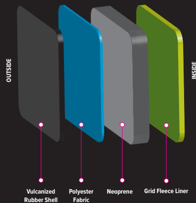
BOOTFOOT UPPER CROSS SECTION
